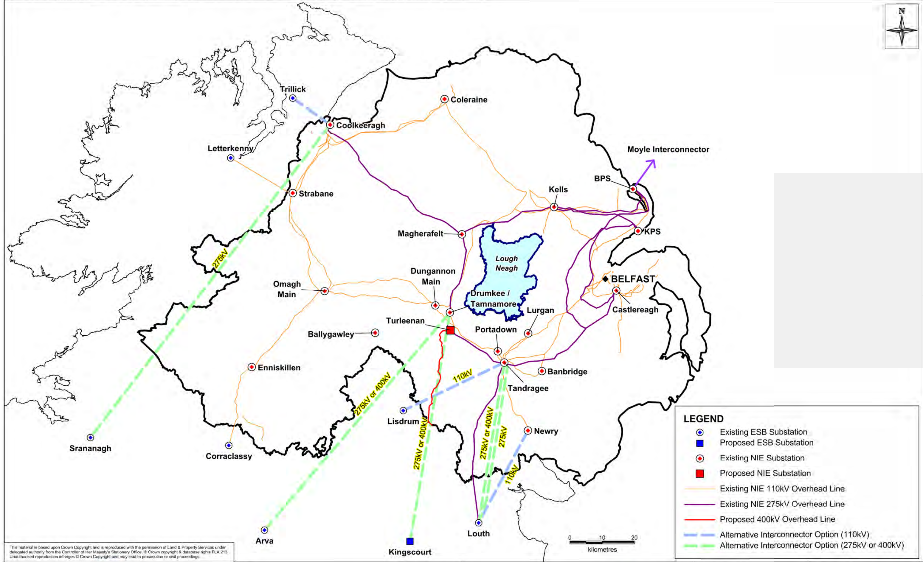
Title: FIGURE 4.2: EXISTING NIE 110kV & 275kV INFRASTRUCTURE AND ALTERNATIVE INTERCONNECTOR OPTIONS
