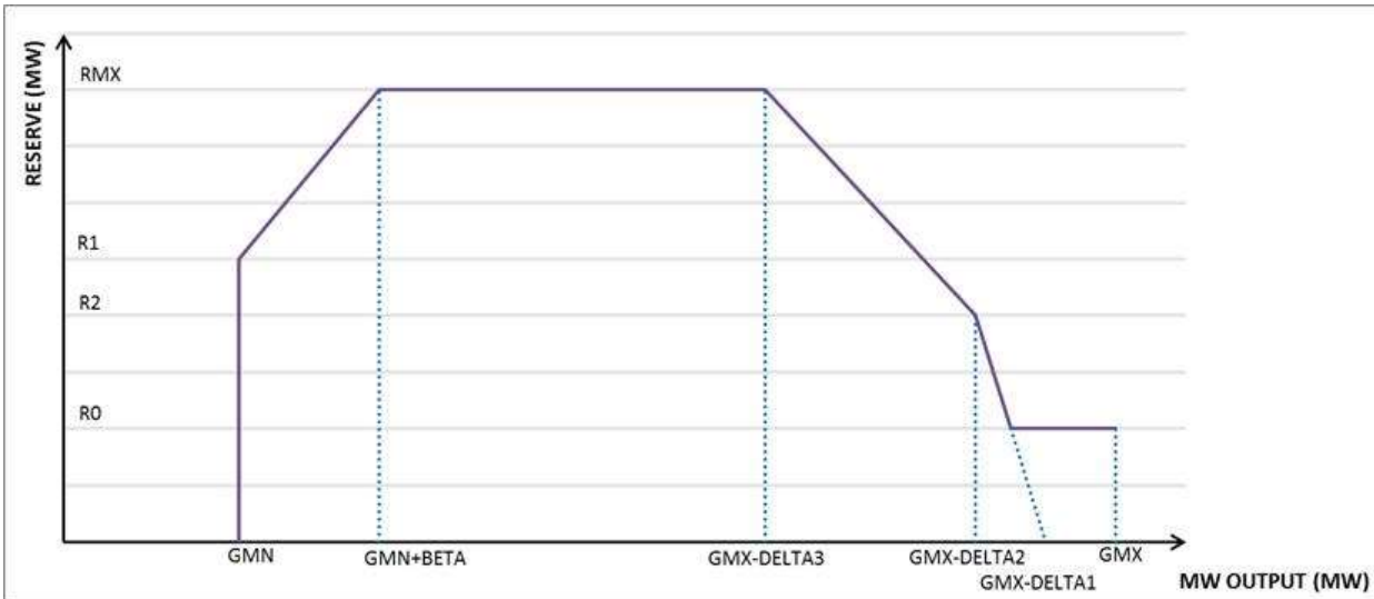
Figure 1 Reserve Characteristic
